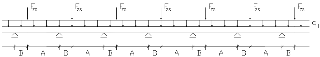
Figure 3.5 Continuous counter batten under constant line loads from actions on the roof plane q_{\perp} and concentrated loads from tensile screws F_{zs}
