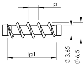
Secondary thread
