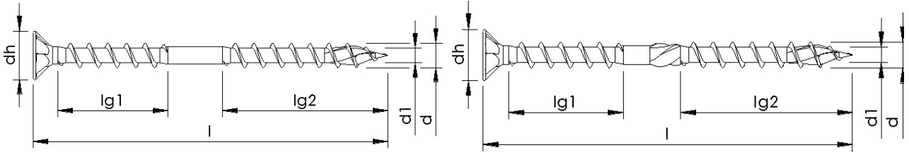
Secondary thread without variation, without shank ribs, with milling ribs
