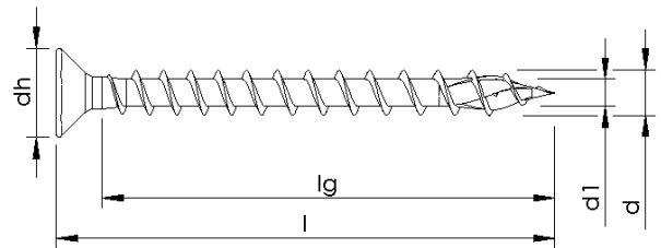
Full thread with variation, with milling ribs
