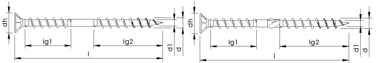
Secondary thread without variation, without shank ribs, with toothed tip
